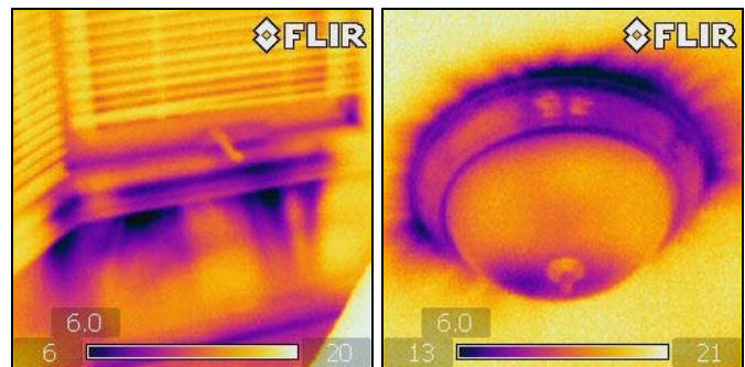
Above ▲ Air infiltration around windows and light fixture. Images taken in conjunction with a blower door test.
